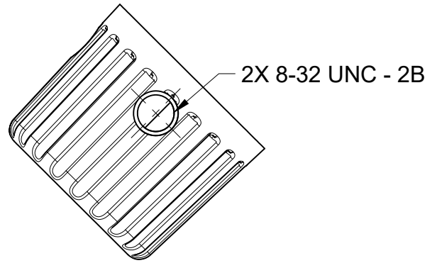
VIEW A-A SCALE 2:1
